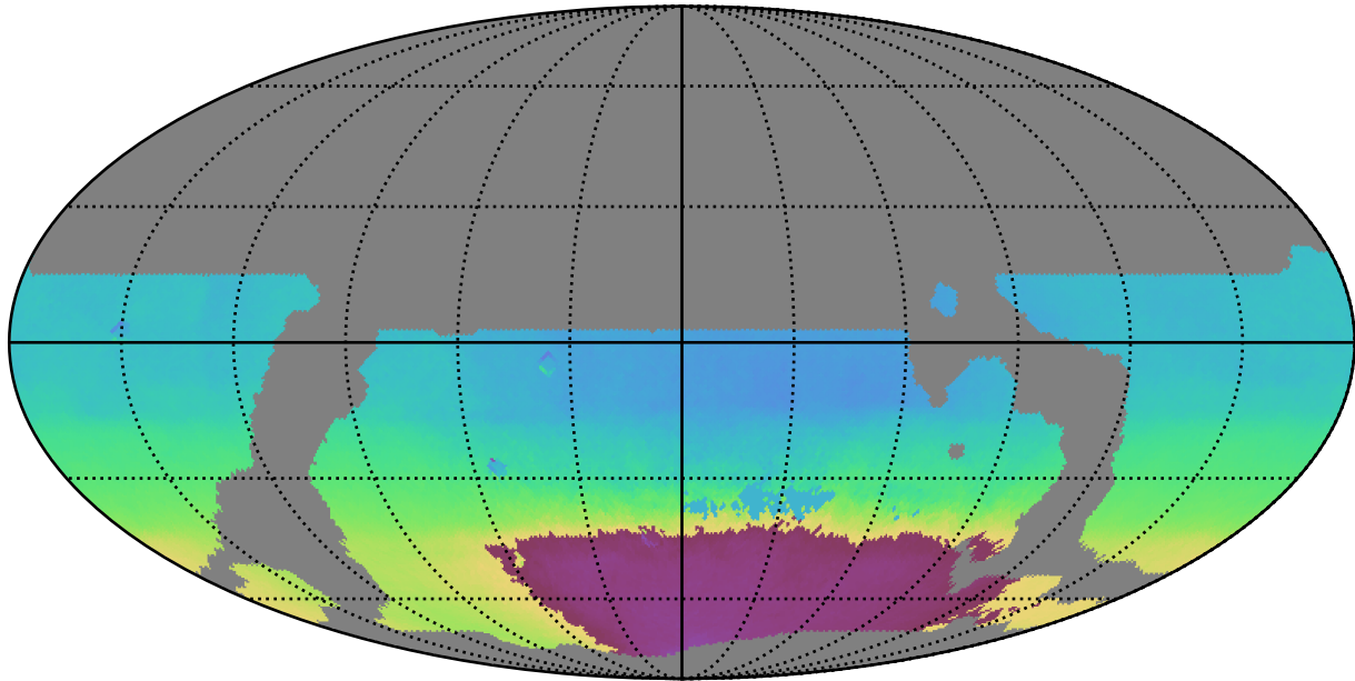
weather_cloudso14v3.4_10yrs WFD all bands: AngleMean rotSkyPos
