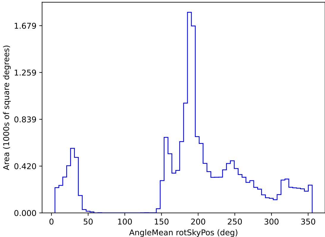
weather_cloudso14v3.4_10yrs WFD all bands: AngleMean rotSkyPos
