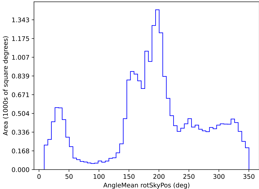
weather_cloudso14v3.4_10yrs All sky u band: AngleMean rotSkyPos
