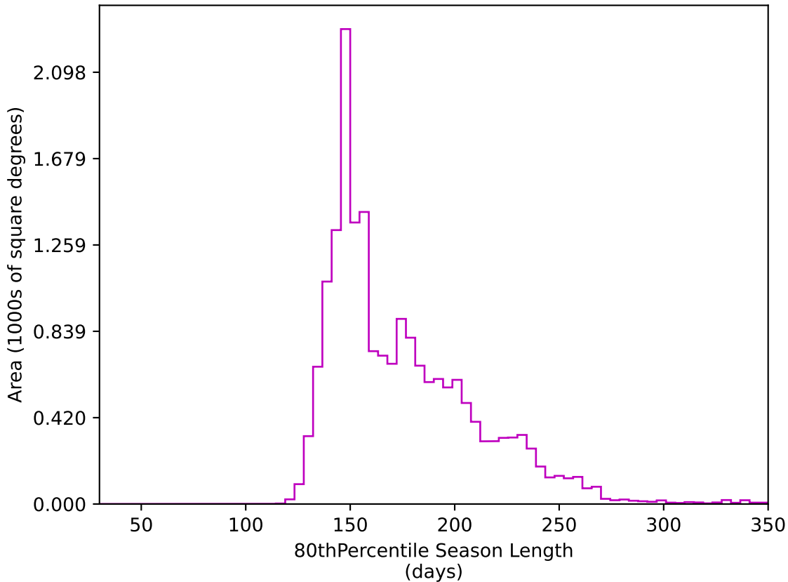
weather_cloudso14v3.4_10yrs WFD z band: 80thPercentile Season Length
