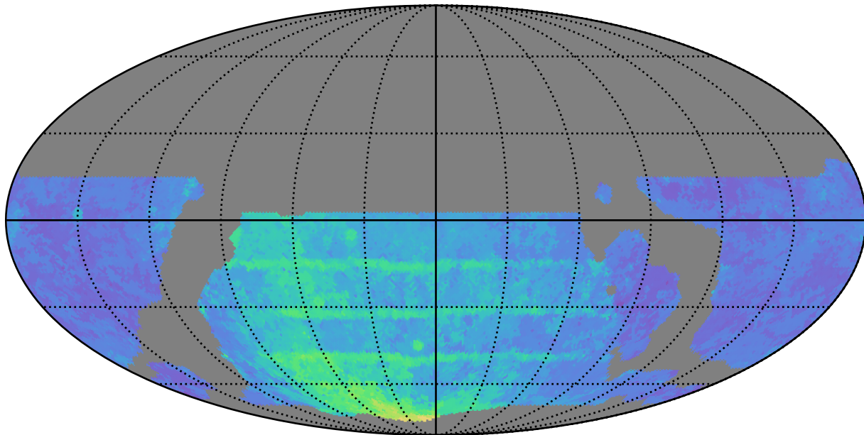
weather_cloudso14v3.4_10yrs WFD y band: 80thPercentile Season Length
