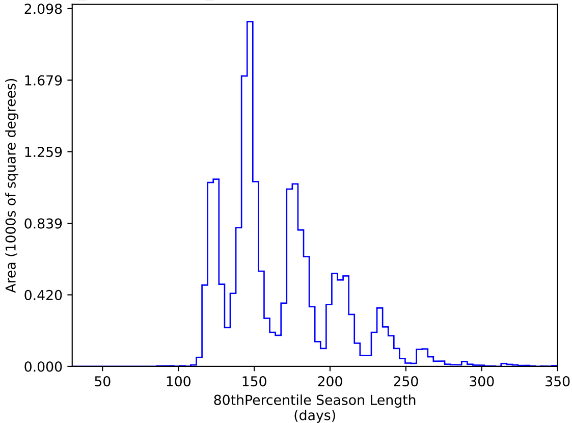
weather_cloudso14v3.4_10yrs WFD y band: 80thPercentile Season Length
