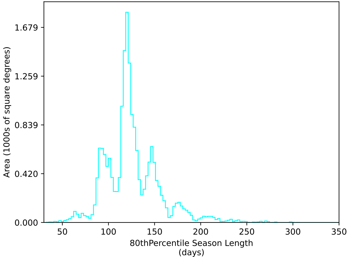
weather_cloudso14v3.4_10yrs WFD u band: 80thPercentile Season Length
