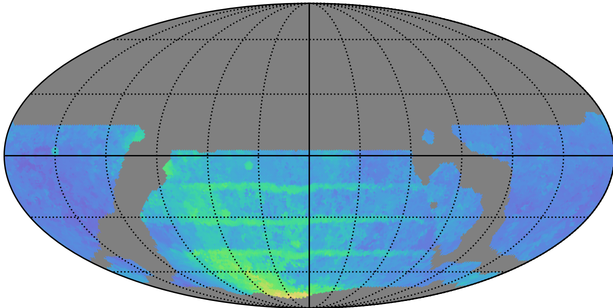
weather_cloudso14v3.4_10yrs WFD r band: 80thPercentile Season Length
