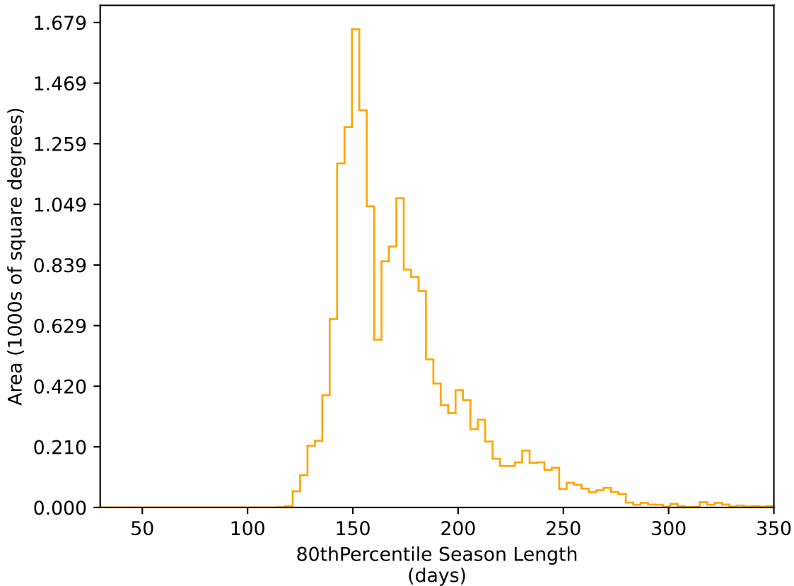
weather_cloudso14v3.4_10yrs WFD r band: 80thPercentile Season Length
