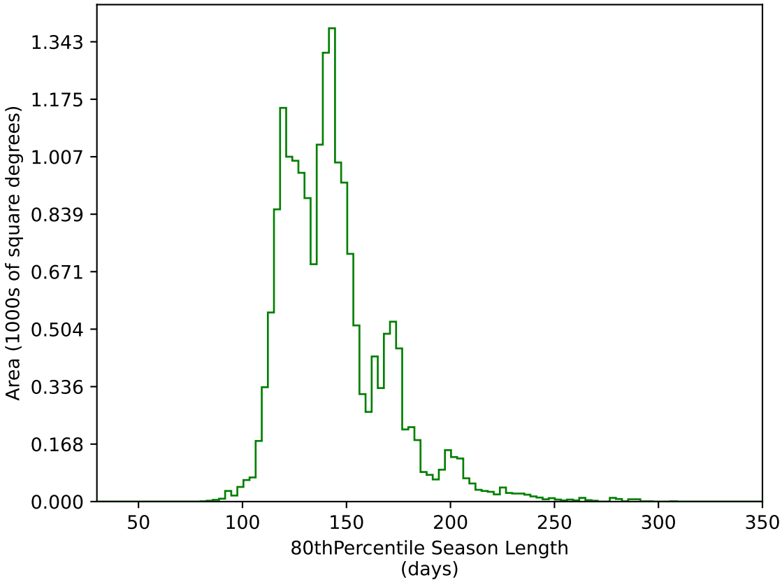
weather_cloudso14v3.4_10yrs WFD g band: 80thPercentile Season Length
