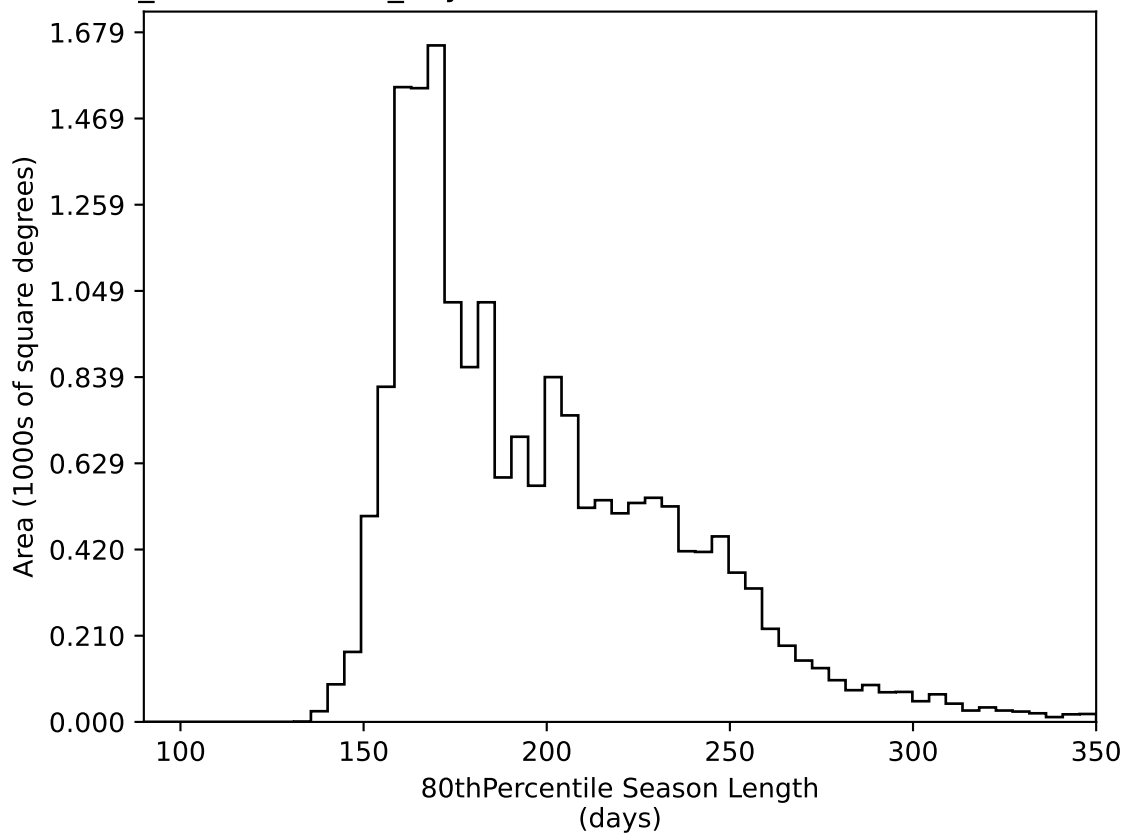
weather_cloudso14v3.4_10yrs WFD all bands: 80thPercentile Season Length
