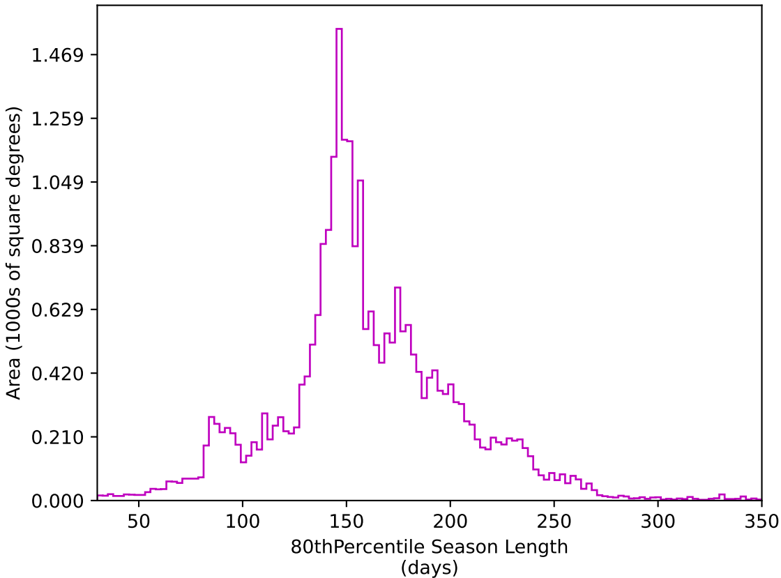
weather_cloudso14v3.4_10yrs All sky z band: 80thPercentile Season Length
