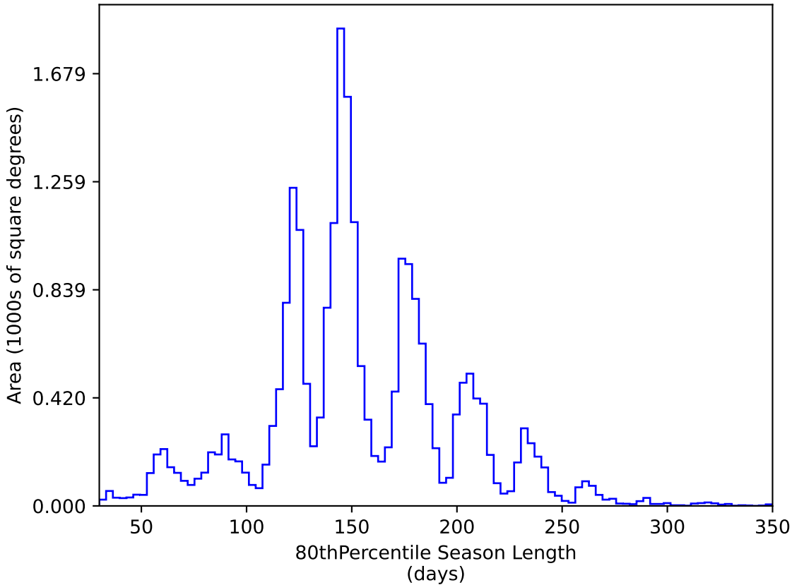
weather_cloudso14v3.4_10yrs All sky y band: 80thPercentile Season Length
