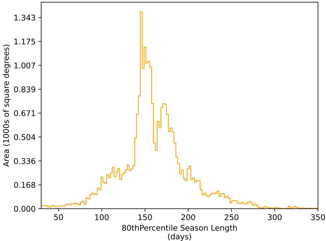
weather_cloudso14v3.4_10yrs All sky r band: 80thPercentile Season Length
