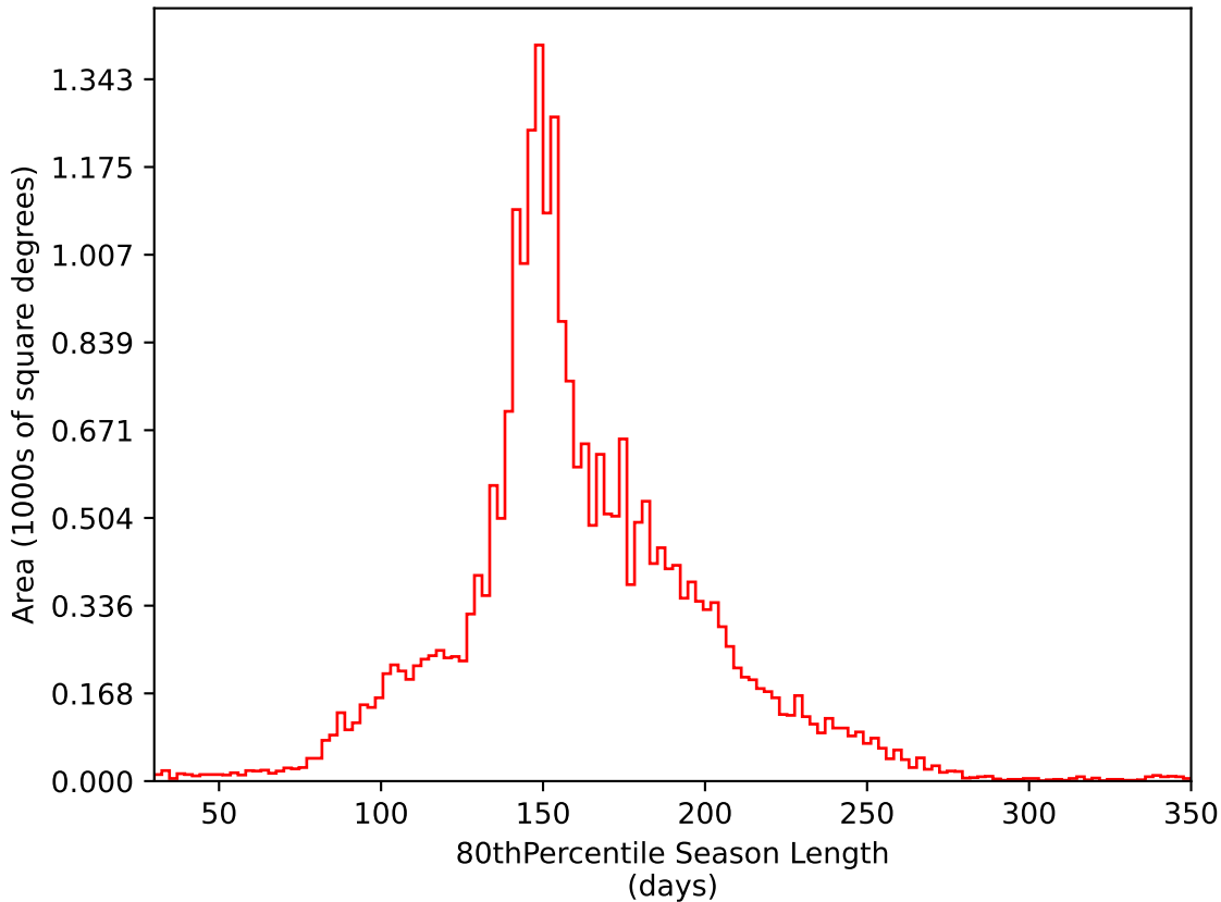
weather_cloudso14v3.4_10yrs All sky i band: 80thPercentile Season Length
