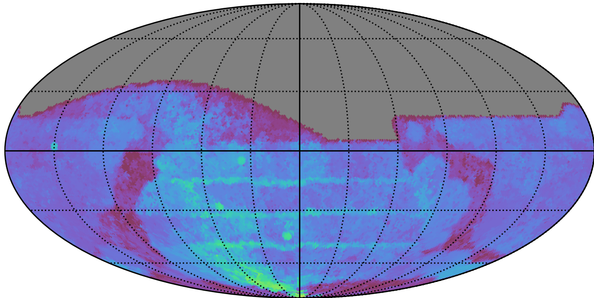
weather_cloudso14v3.4_10yrs All sky g band: 80thPercentile Season Length
