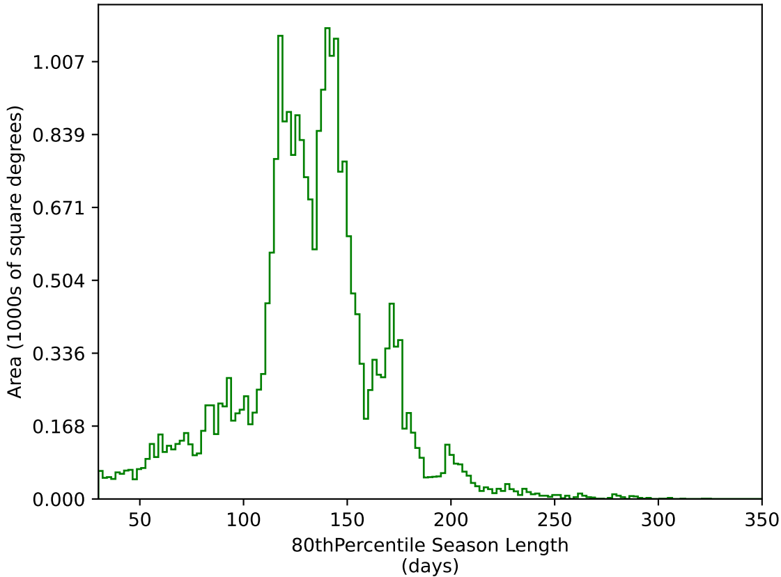
weather_cloudso14v3.4_10yrs All sky g band: 80thPercentile Season Length
