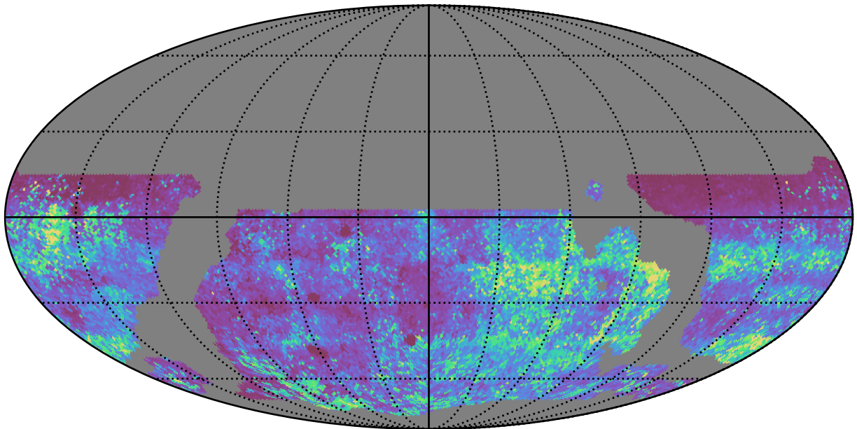
weather_cloudso14v3.4_10yrs WFD zy bands: 75th Percentile Intranight Timespan
