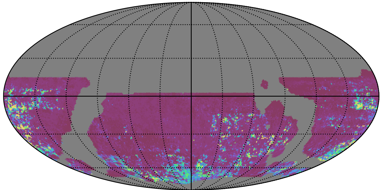
weather_cloudso14v3.4_10yrs WFD z band: 75th Percentile Intranight Timespan
