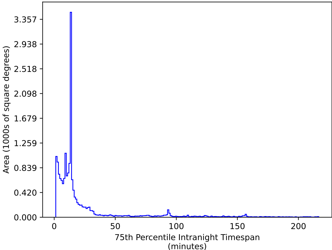
weather_cloudso14v3.4_10yrs WFD z band: 75th Percentile Intranight Timespan
