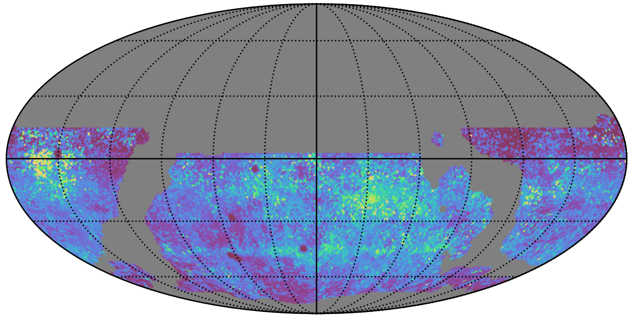
weather_cloudso14v3.4_10yrs WFD y band: 75th Percentile Intranight Timespan
