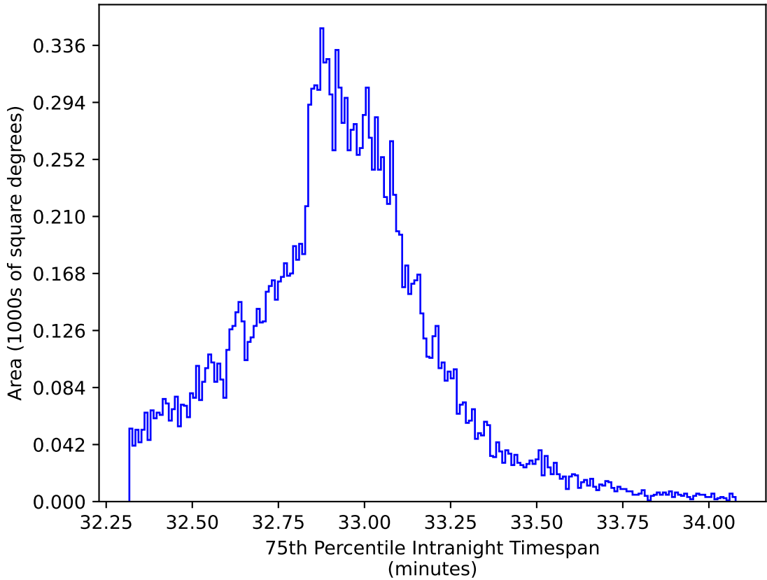
weather_cloudso14v3.4_10yrs WFD y band: 75th Percentile Intranight Timespan
