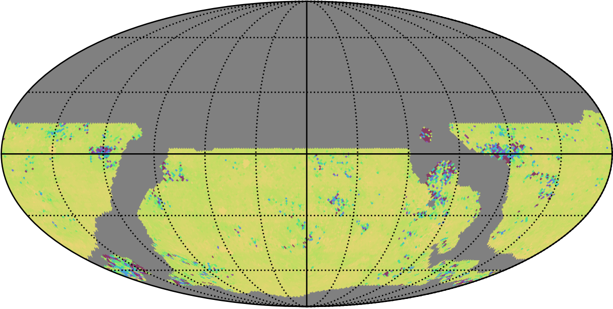
weather_cloudso14v3.4_10yrs WFD ug bands: 75th Percentile Intranight Timespan
