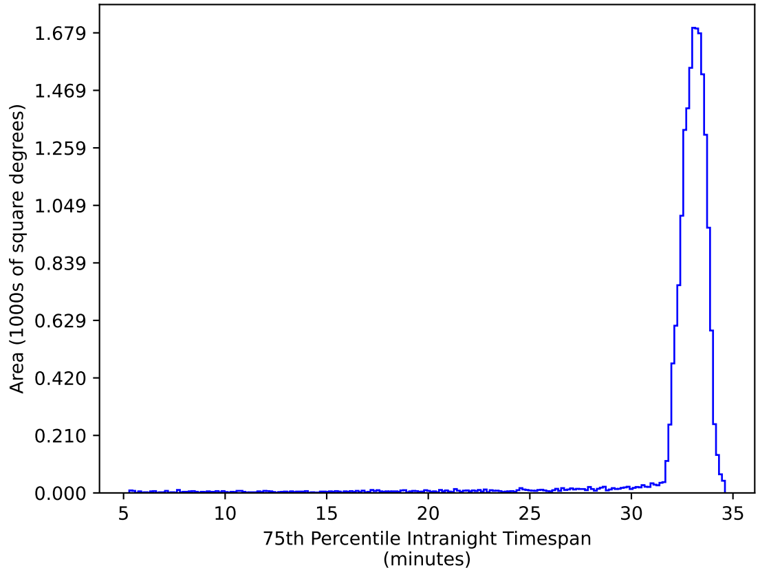
weather_cloudso14v3.4_10yrs WFD ug bands: 75th Percentile Intranight Timespan
