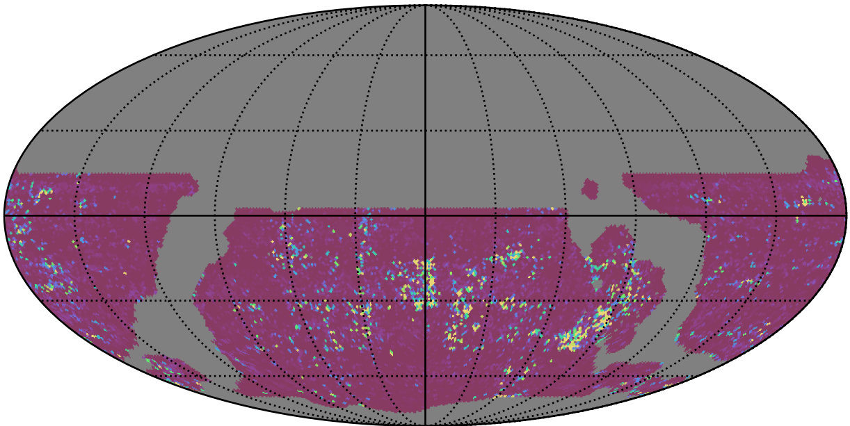
weather_cloudso14v3.4_10yrs WFD u band: 75th Percentile Intranight Timespan
