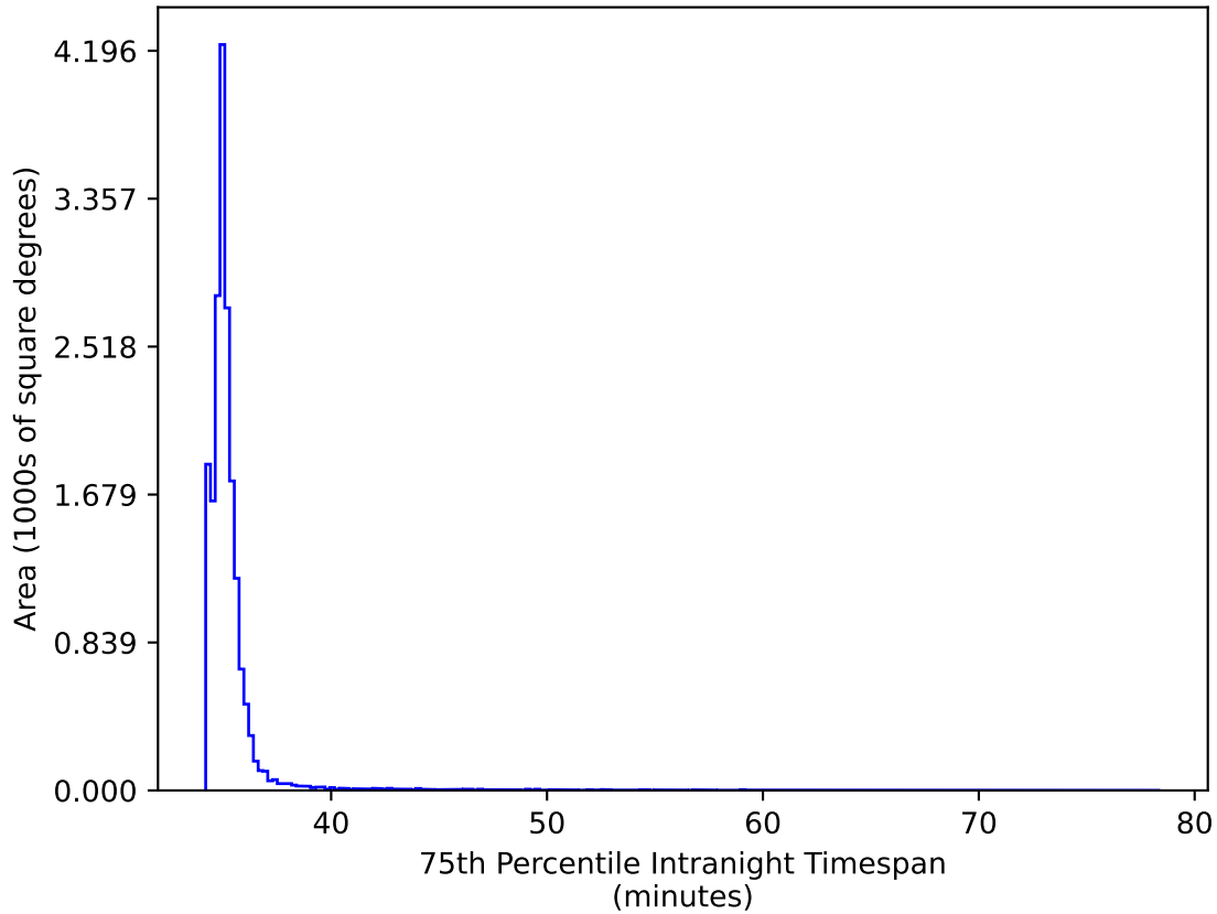
weather_cloudso14v3.4_10yrs WFD ri bands: 75th Percentile Intranight Timespan
