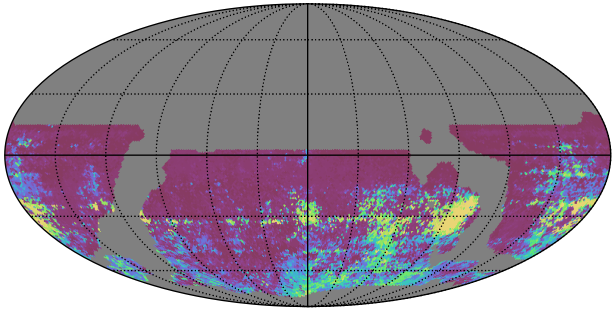
weather_cloudso14v3.4_10yrs WFD r band: 75th Percentile Intranight Timespan
