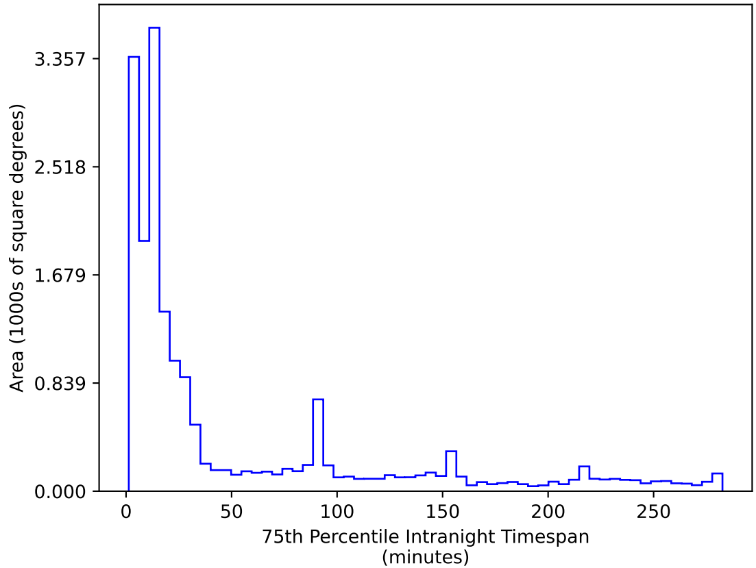
weather_cloudso14v3.4_10yrs WFD r band: 75th Percentile Intranight Timespan
