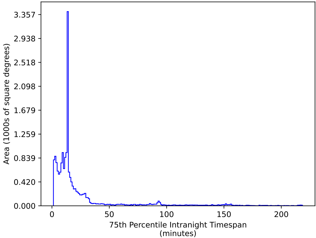
weather_cloudso14v3.4_10yrs WFD i band: 75th Percentile Intranight Timespan
