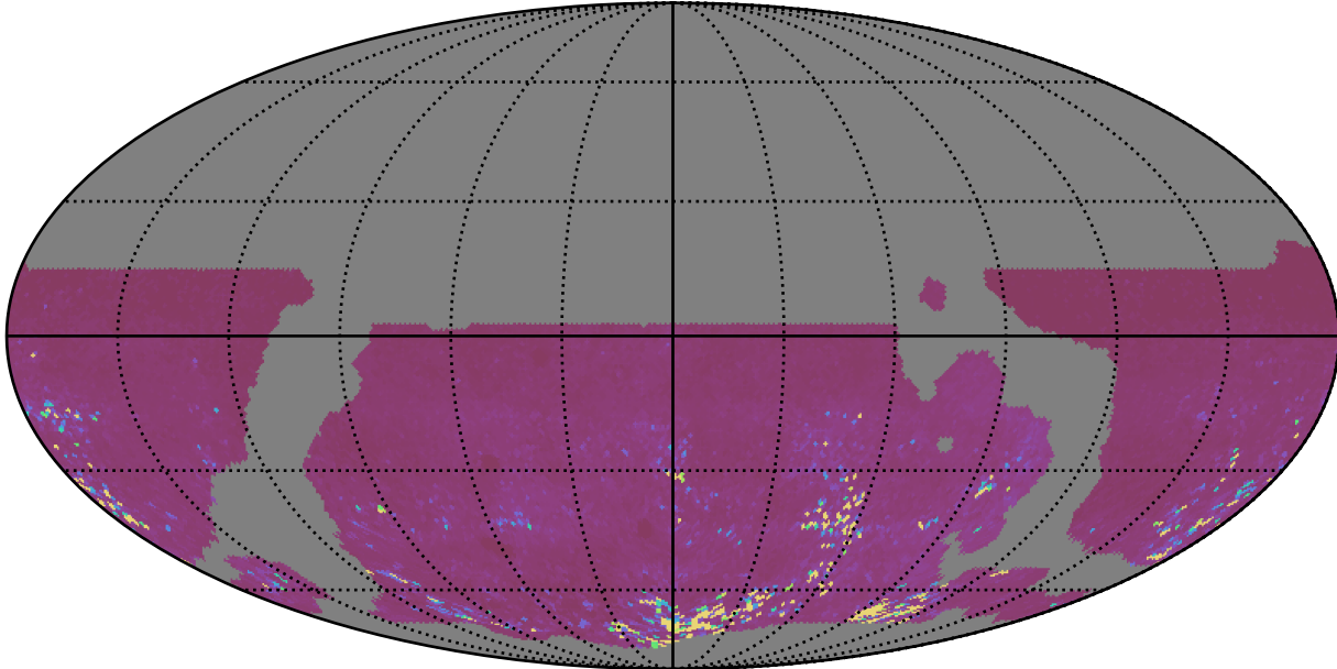
weather_cloudso14v3.4_10yrs WFD gr bands: 75th Percentile Intranight Timespan
