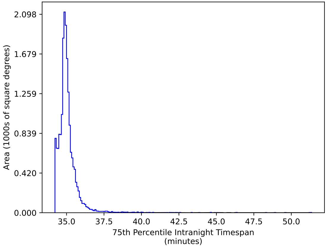
weather_cloudso14v3.4_10yrs WFD gr bands: 75th Percentile Intranight Timespan
