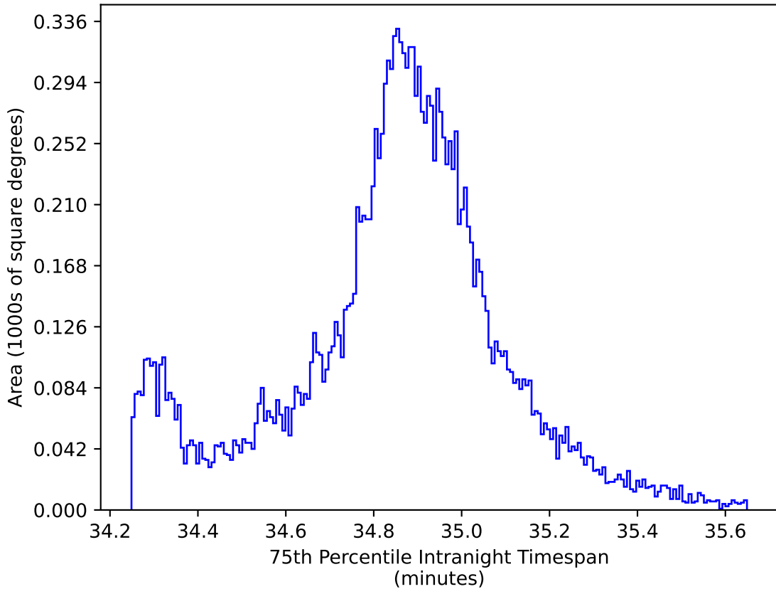
weather_cloudso14v3.4_10yrs WFD: 75th Percentile Intranight Timespan
