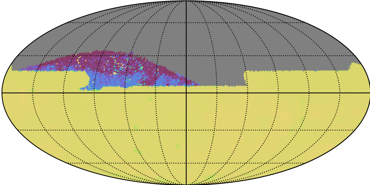
weather_cloudso14v3.4_10yrs All sky zy bands: 75th Percentile Intranight Timespan
