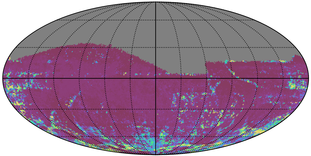
weather_cloudso14v3.4_10yrs All sky z band: 75th Percentile Intranight Timespan
