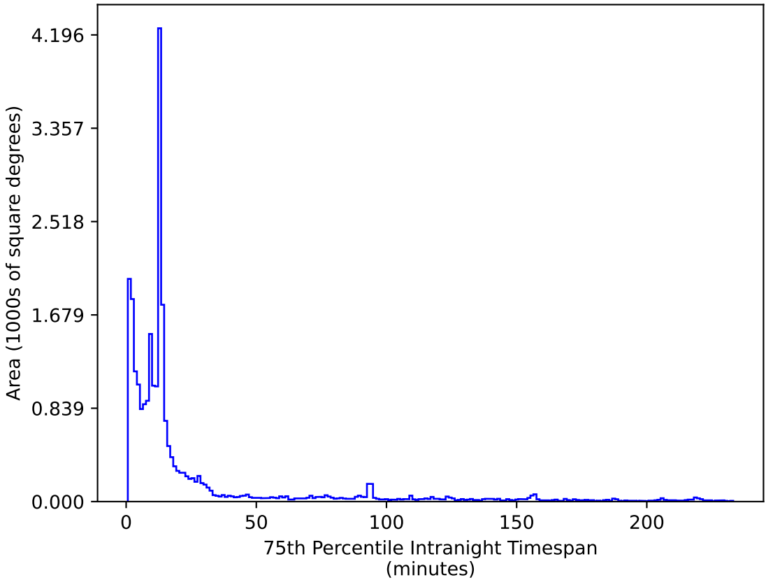
weather_cloudso14v3.4_10yrs All sky z band: 75th Percentile Intranight Timespan
