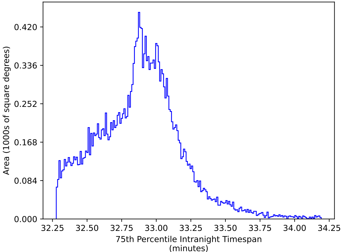
weather_cloudso14v3.4_10yrs All sky y band: 75th Percentile Intranight Timespan
