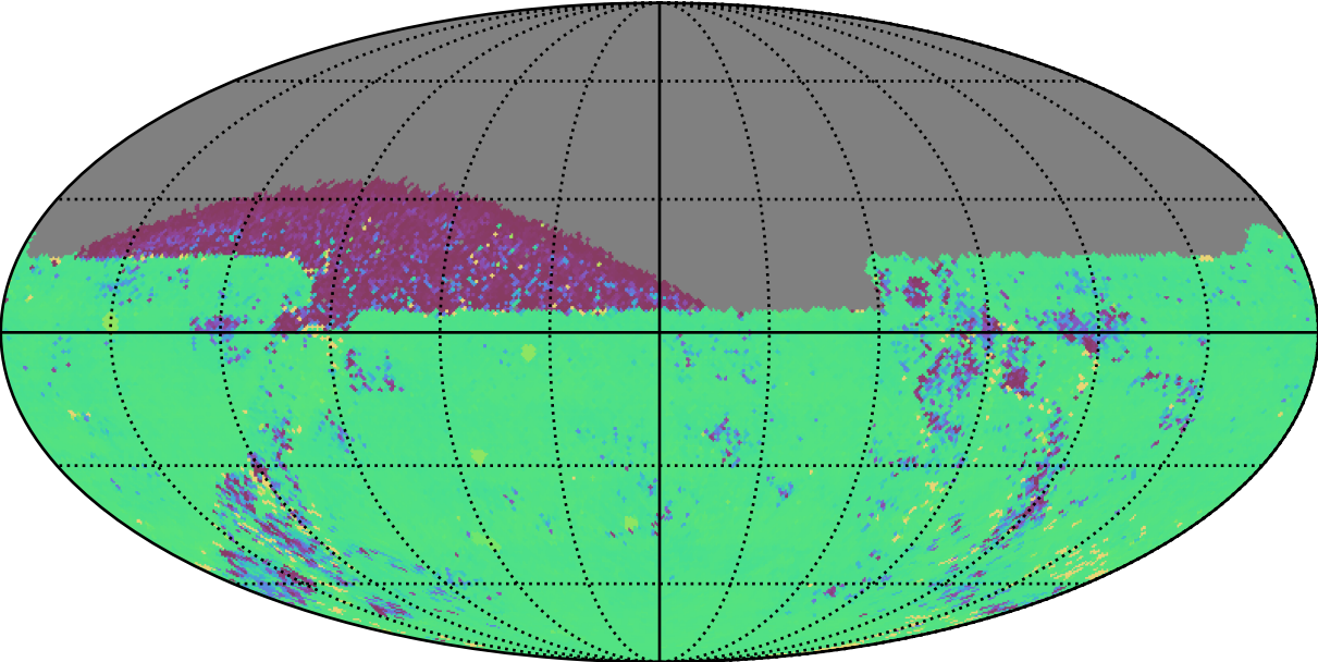
weather_cloudso14v3.4_10yrs All sky ug bands: 75th Percentile Intranight Timespan
