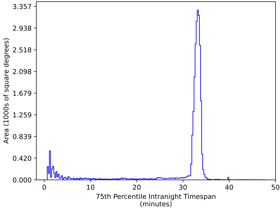
weather_cloudso14v3.4_10yrs All sky ug bands: 75th Percentile Intranight Timespan
