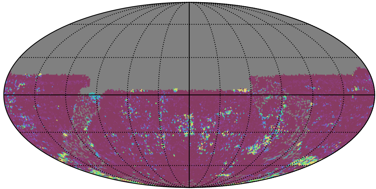
weather_cloudso14v3.4_10yrs All sky u band: 75th Percentile Intranight Timespan
