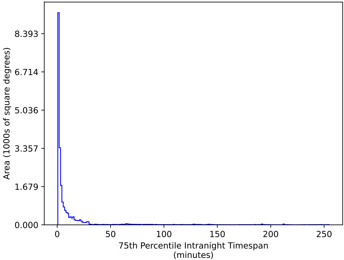
weather_cloudso14v3.4_10yrs All sky u band: 75th Percentile Intranight Timespan
