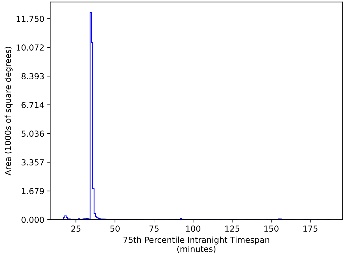
weather_cloudso14v3.4_10yrs All sky ri bands: 75th Percentile Intranight Timespan
