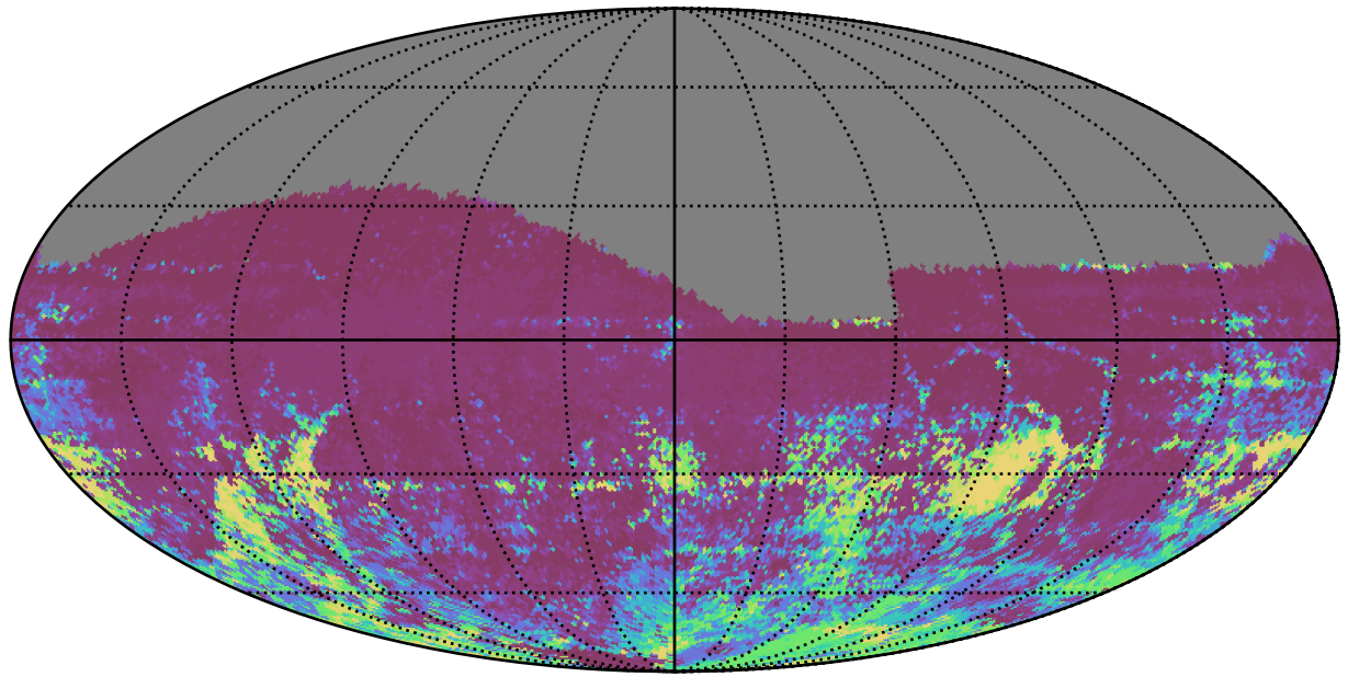
weather_cloudso14v3.4_10yrs All sky r band: 75th Percentile Intranight Timespan
