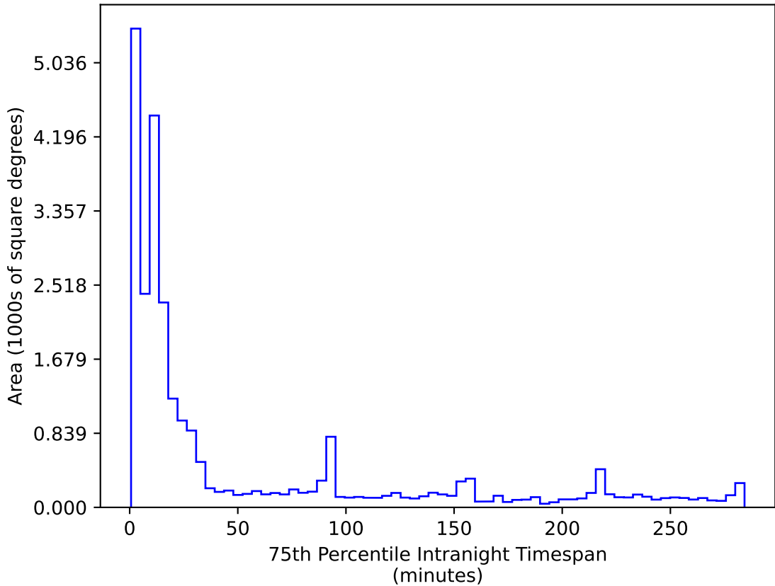
weather_cloudso14v3.4_10yrs All sky r band: 75th Percentile Intranight Timespan
