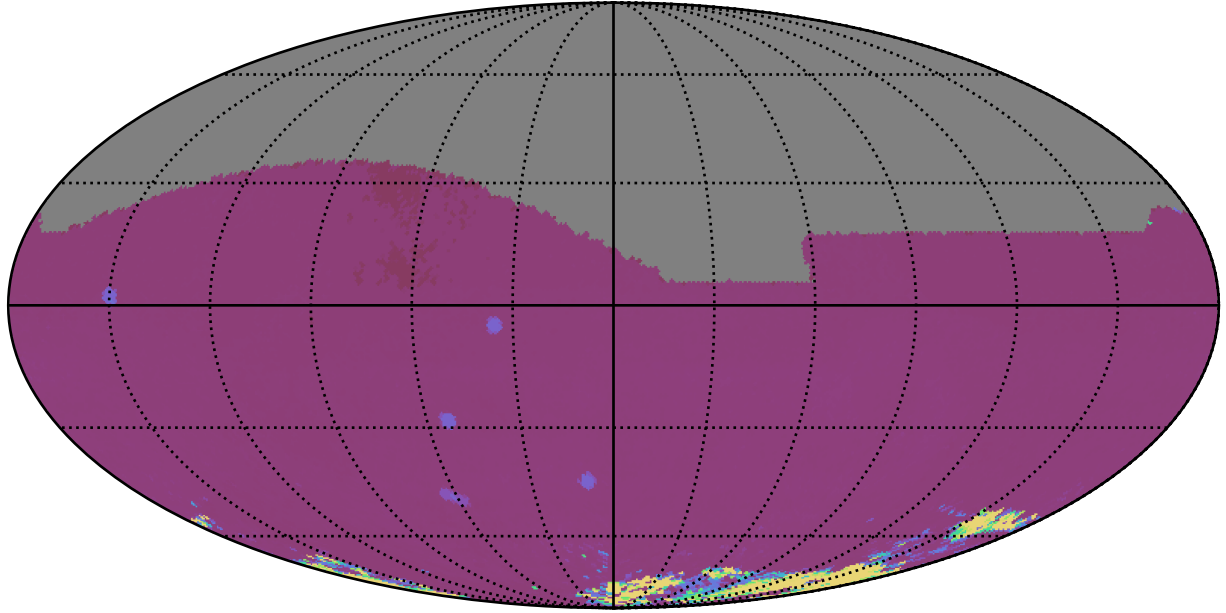
weather_cloudso14v3.4_10yrs All sky iz bands: 75th Percentile Intranight Timespan
