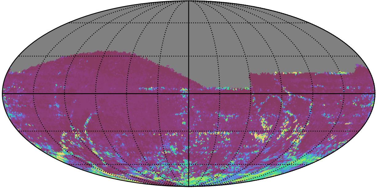
weather_cloudso14v3.4_10yrs All sky i band: 75th Percentile Intranight Timespan
