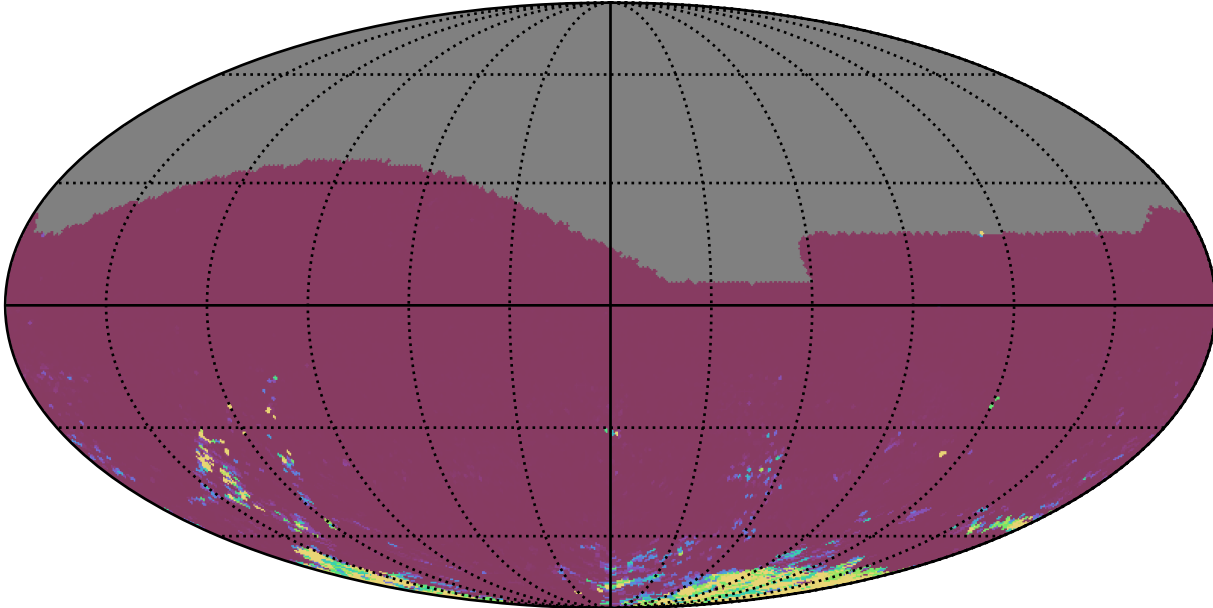
weather_cloudso14v3.4_10yrs All sky gr bands: 75th Percentile Intranight Timespan
