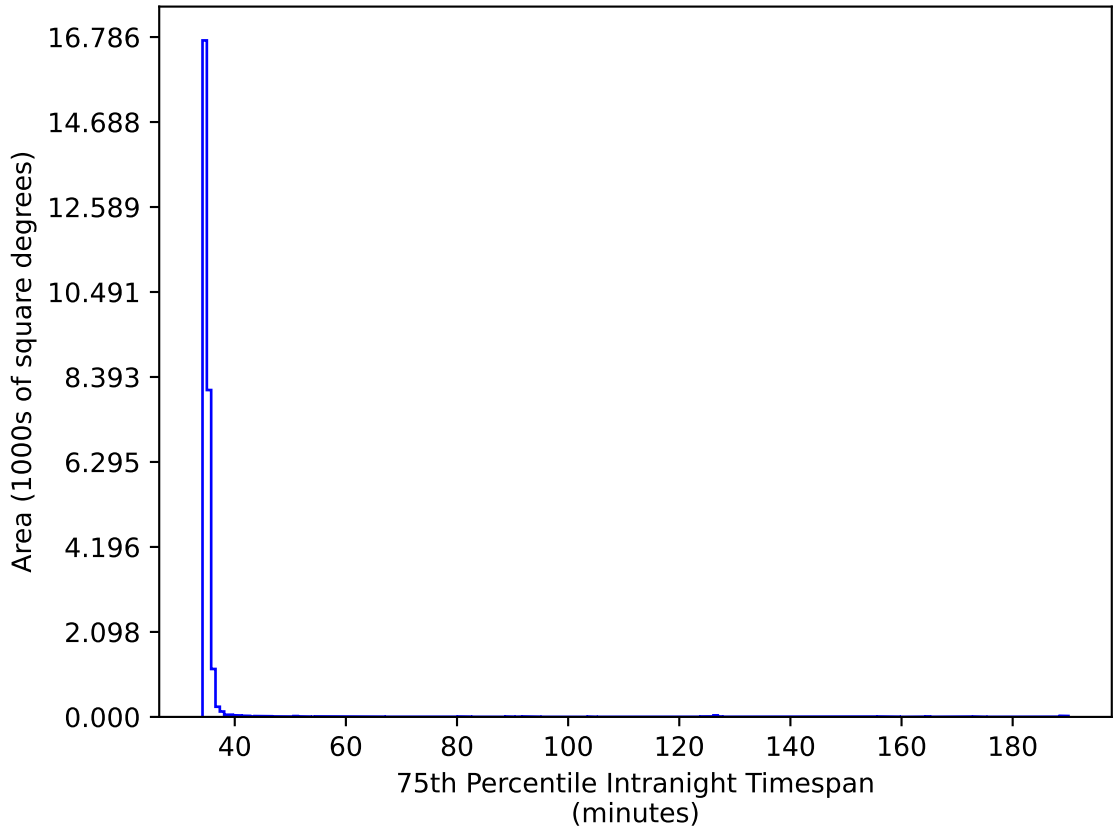
weather_cloudso14v3.4_10yrs All sky gr bands: 75th Percentile Intranight Timespan
