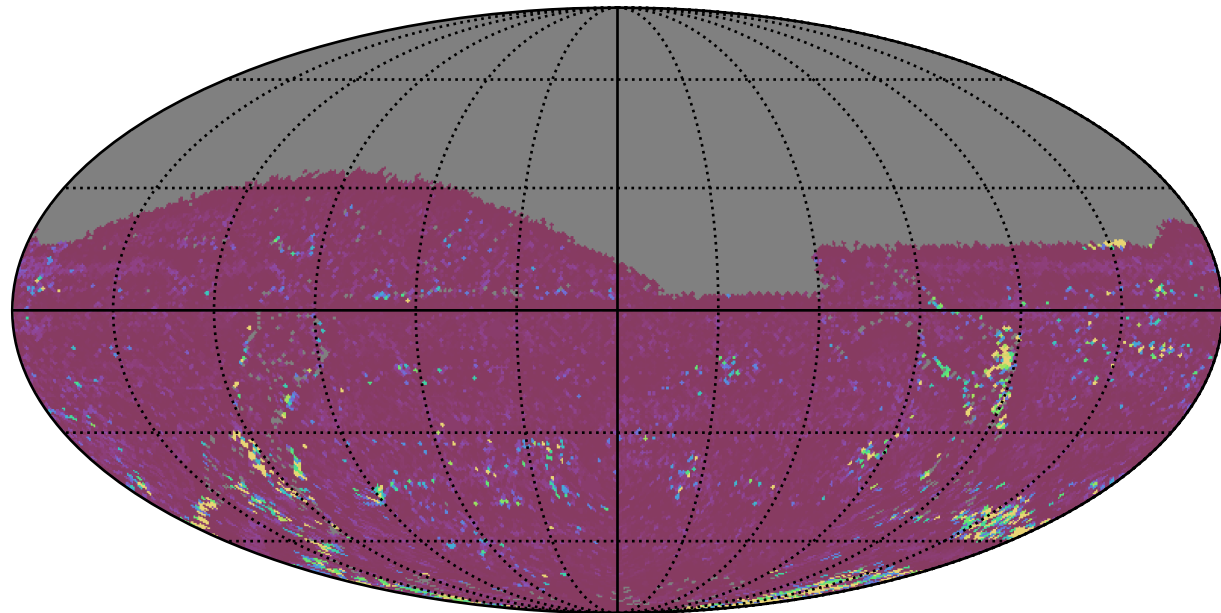
weather_cloudso14v3.4_10yrs All sky g band: 75th Percentile Intranight Timespan
