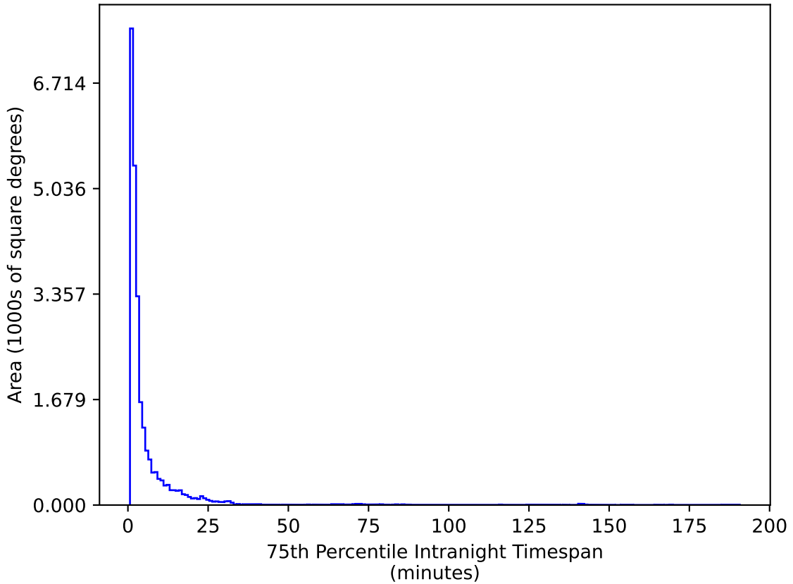
weather_cloudso14v3.4_10yrs All sky g band: 75th Percentile Intranight Timespan
