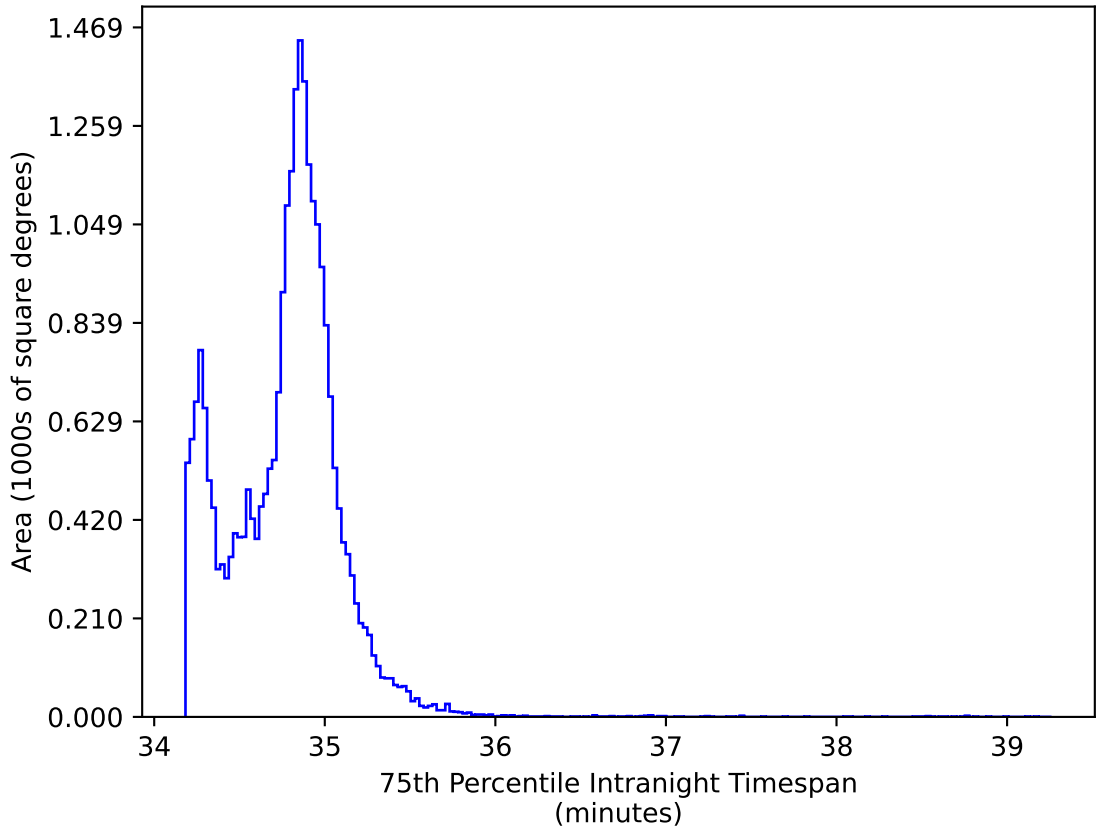
weather_cloudso14v3.4_10yrs All sky all bands: 75th Percentile Intranight Timespan
